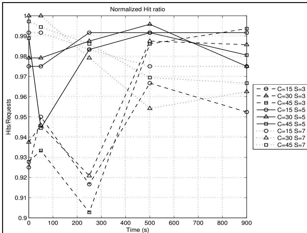
Figure 13. Hit ratio, dependence on the pause time
