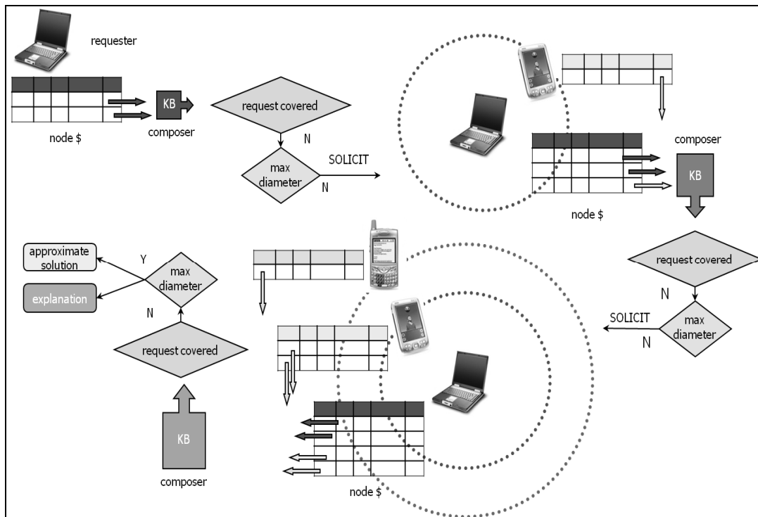
Figure 8. The solicting mechanism
