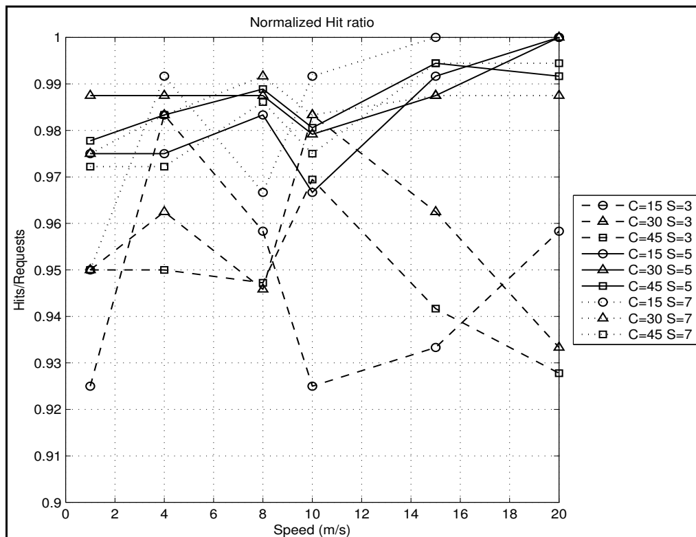
Figure 14. Hit ratio, dependence on the maximum speed
