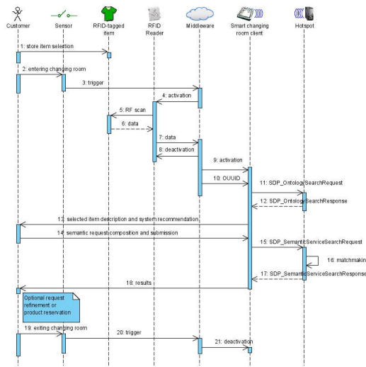
Figure 5: Sequence diagram of a basic use case in our application
