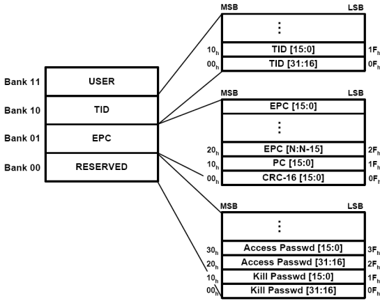
Figure 3: Memory model for adopted UHF RFID tags (from EPCglobal)
