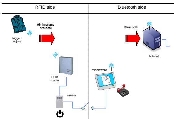
Figure 1: Proposed framework components
