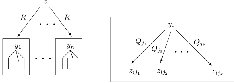
Fig. 3.1. The AND-tree structure of the tableau obtained by applying rules for \sqcap and \exists R.C to (D_1 \sqcap D_2 \sqcap D_3)(x) . Applying rule for (\leq 2 R)(x) would lead to several OR-branches (as many as the possible identifications of y 's)
